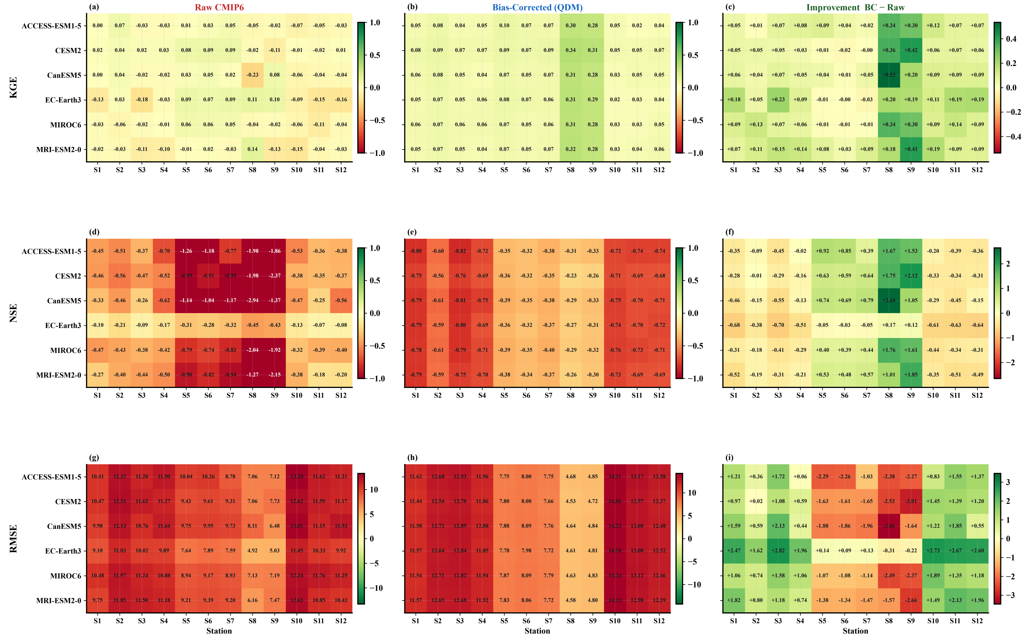
Station-scale performance heatmap — Individual CMIP6 models Raw CMIP6 | Bias-Corrected (QDM) | Improvement (BC – Raw) | Period: 1981–2014
